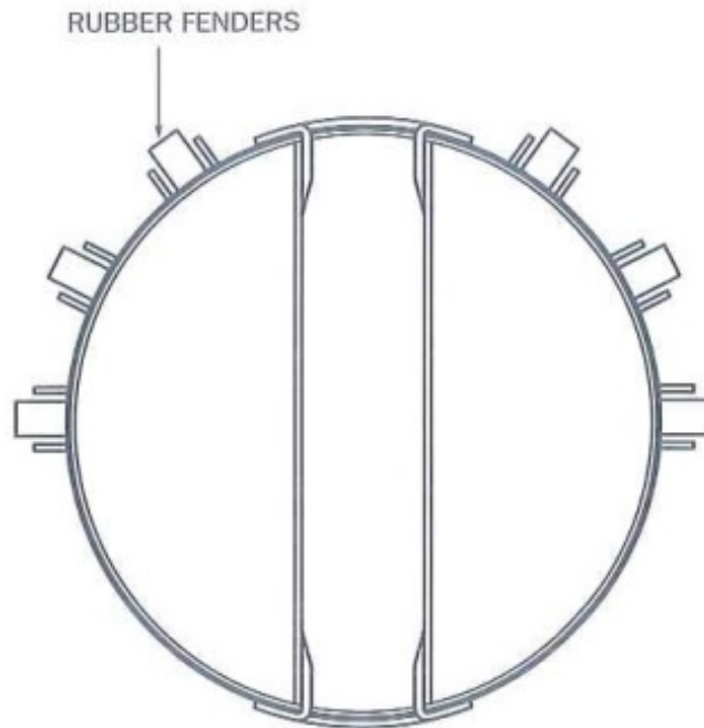
SECTION THROUGH FABRICATED COLLAR
